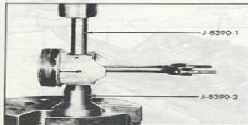
Fig. 9-2 Piston Pin Removal
