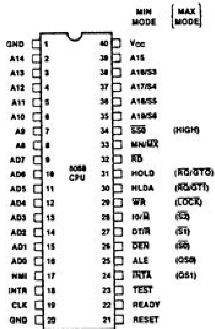
Figure 2. 8088 Pin Configuration
