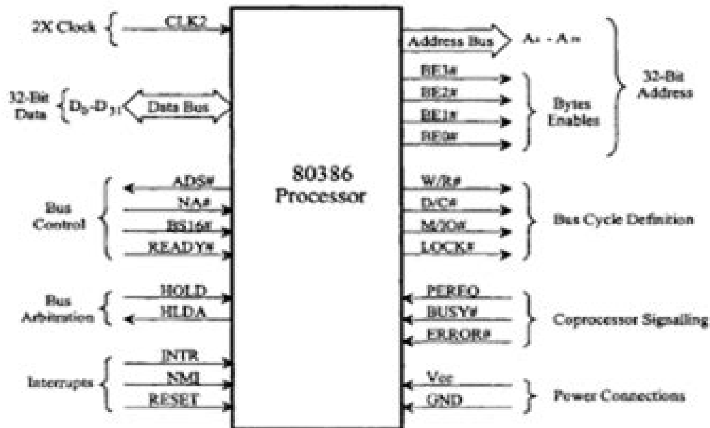
FIGURE 11.2 80386 Functional signal groups
