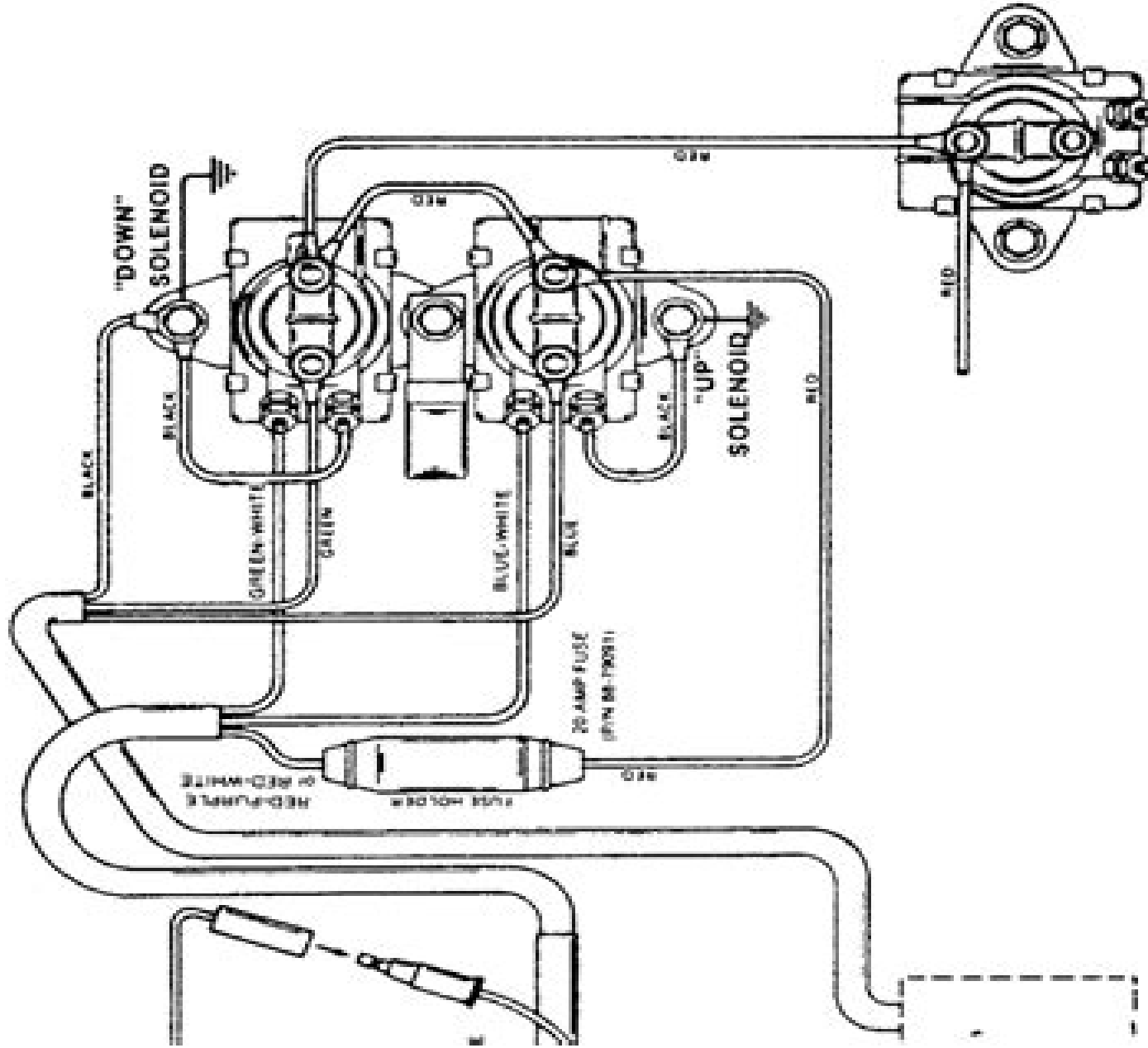
ENGINE STARTER MOTOR SOLENOID
