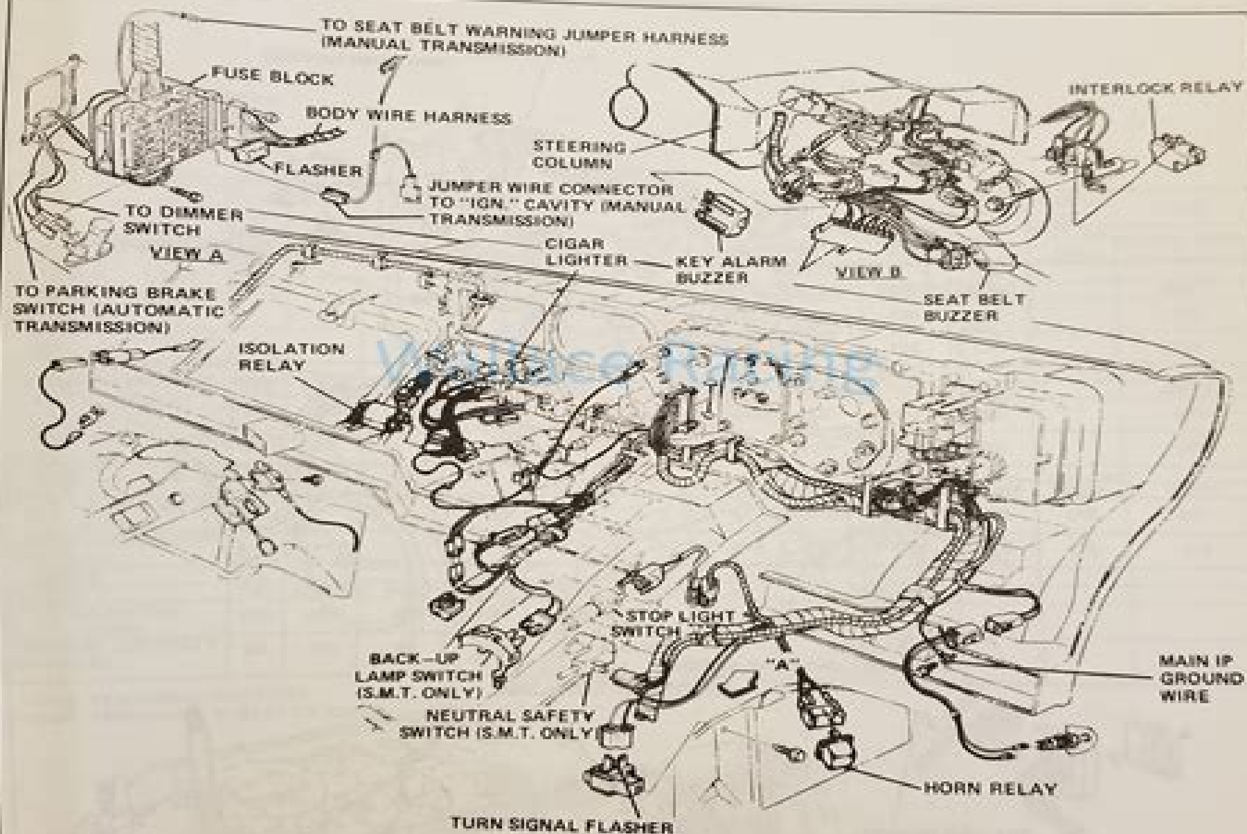
Fig. 12-87 F Series Instrument Panel Wire Harness Installation
