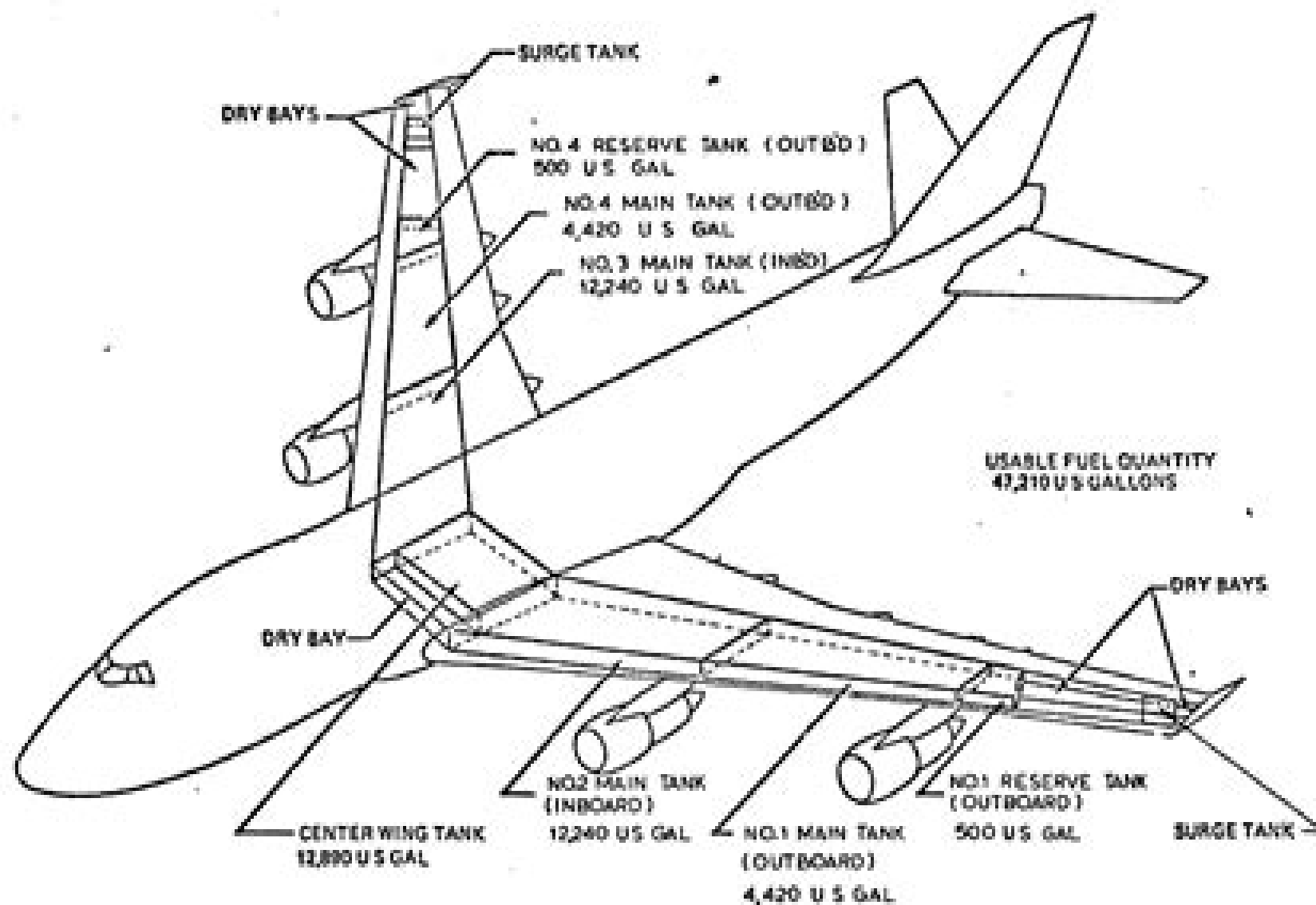
Fig. 1 - Fuel tanks
