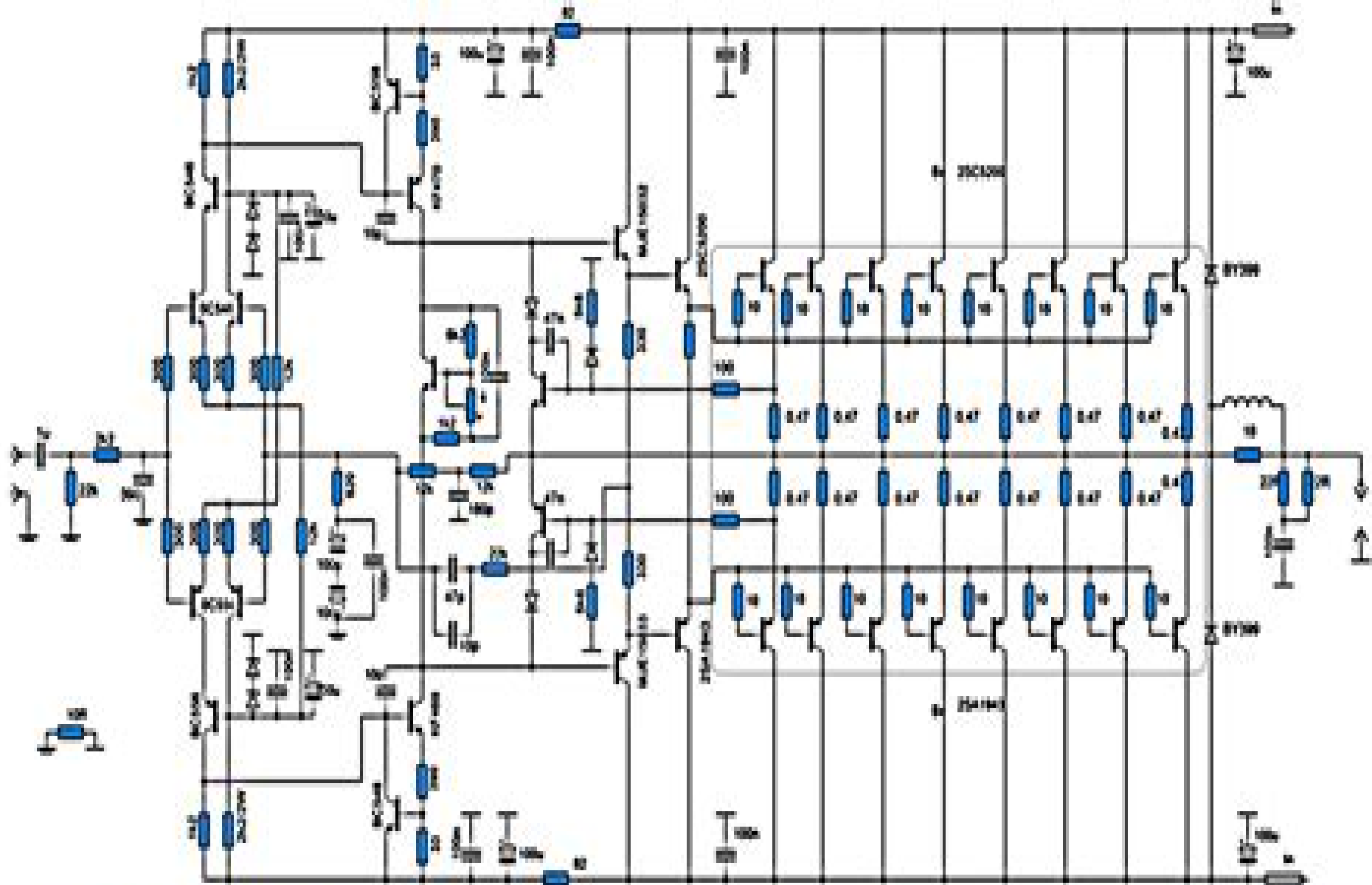
HIGH POWER AMPLIFIER CIRCUIT DIAGRAM
