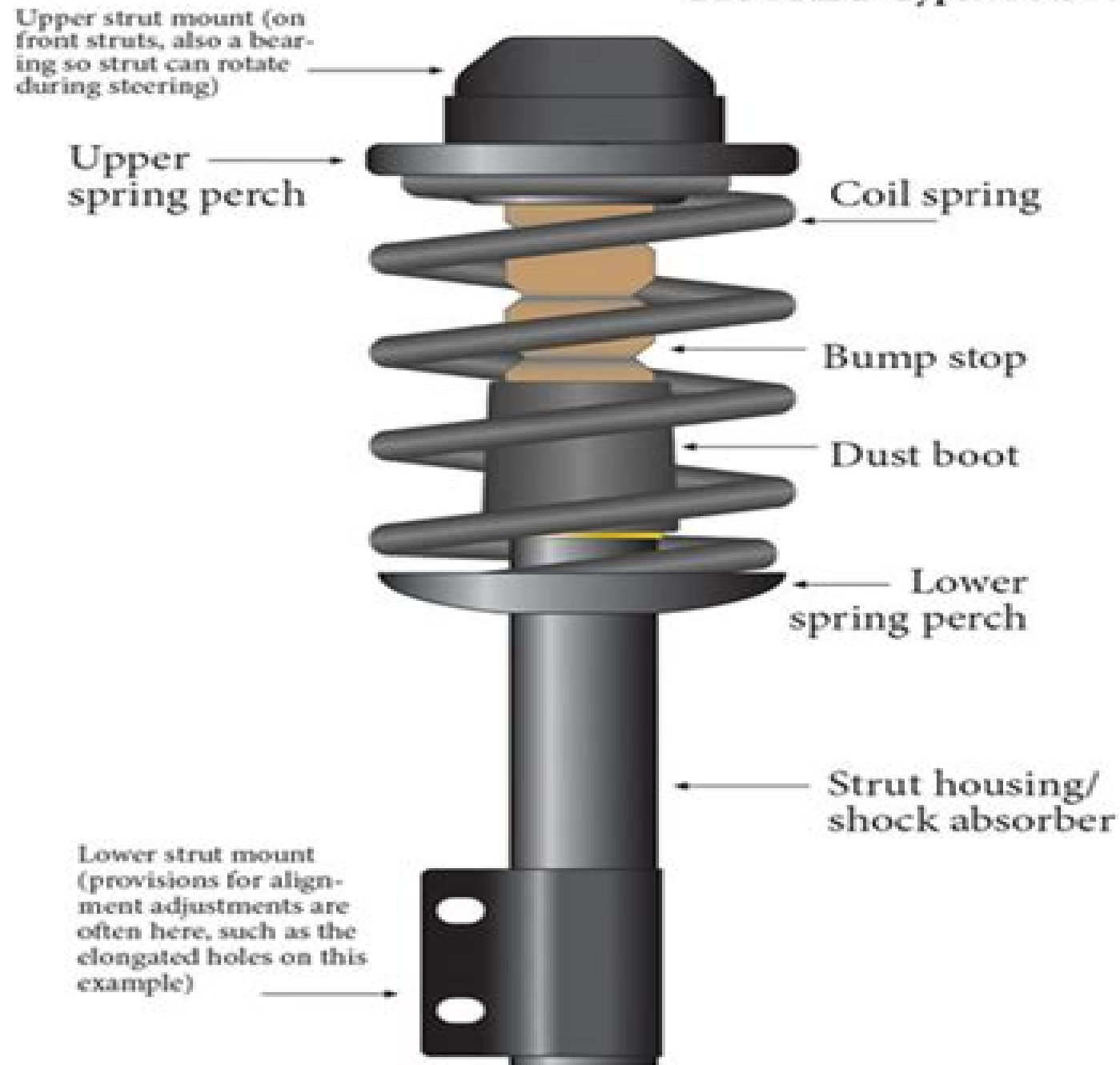
FIGURE 1: Typical Strut
