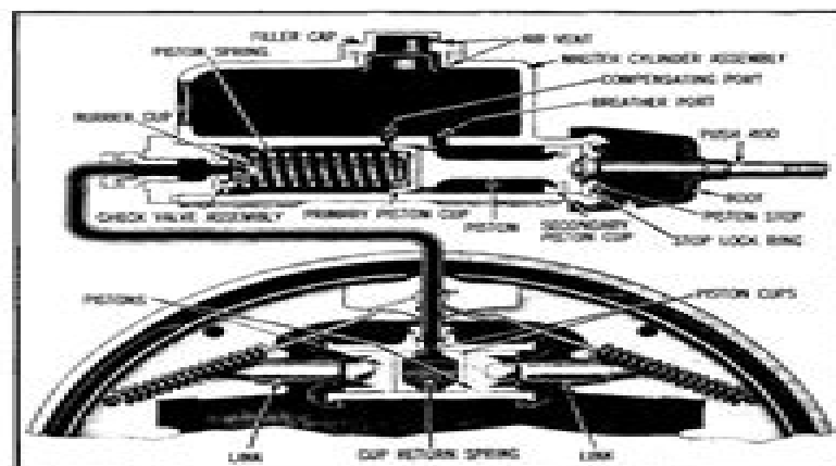
Fig. 5-4 Schematic Diagram of Hydraulic System
