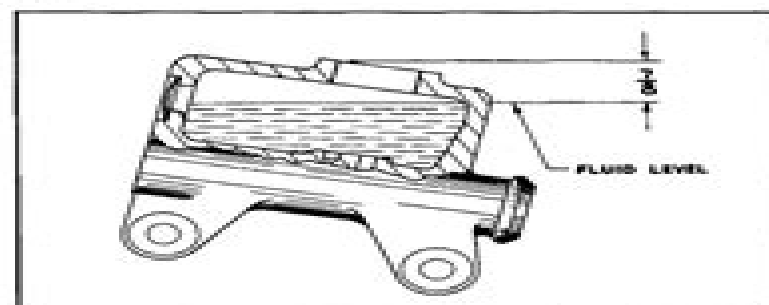
Fig. 5-5 Correct Level in Master Cylinder
