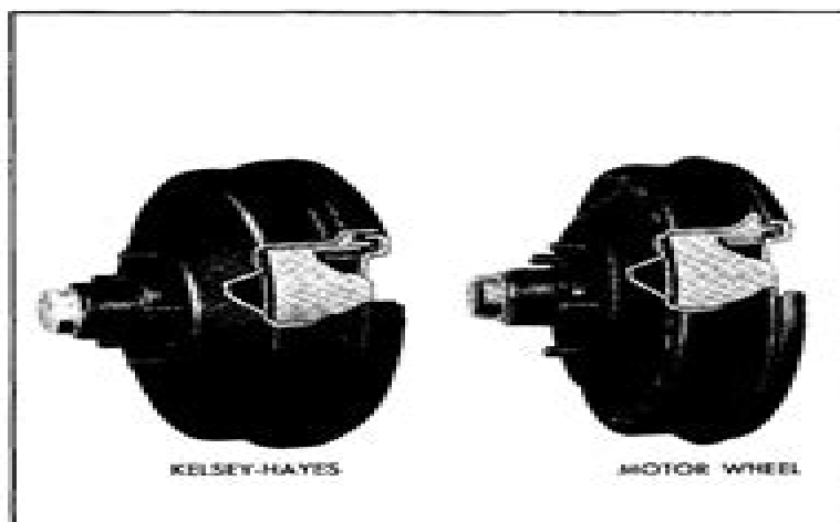
Fig. 5-3 Front Brake Seals
