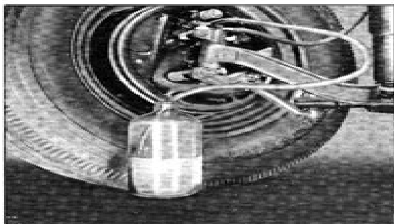
Fig. 9—Bleeding Brake System at Wheel Cylinder
