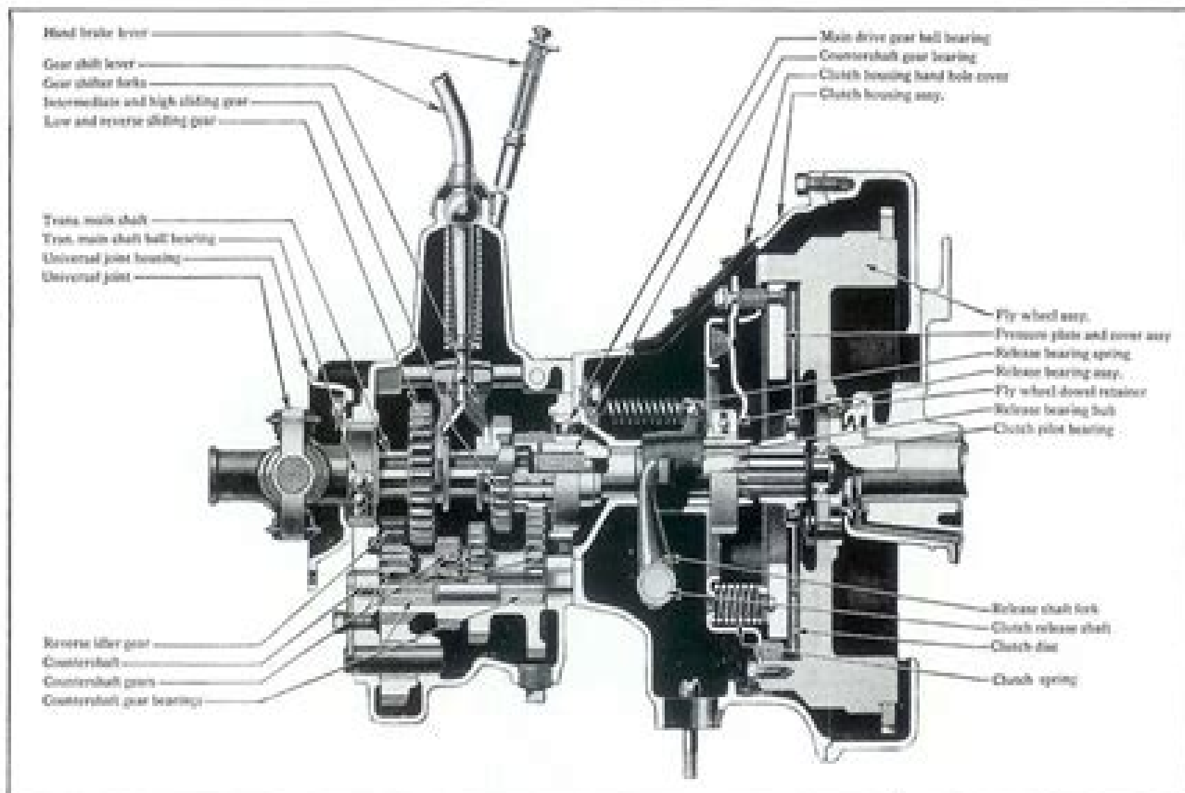
Figure 6 Transmission and Clutch
