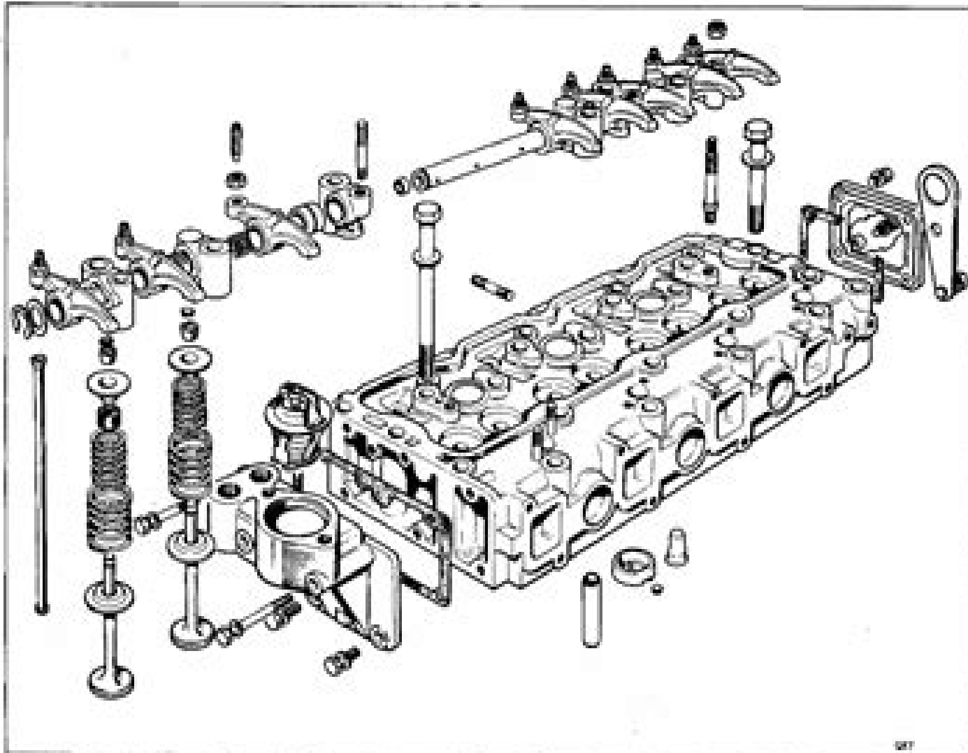
Exploded View of Cylinder Head Assembly
