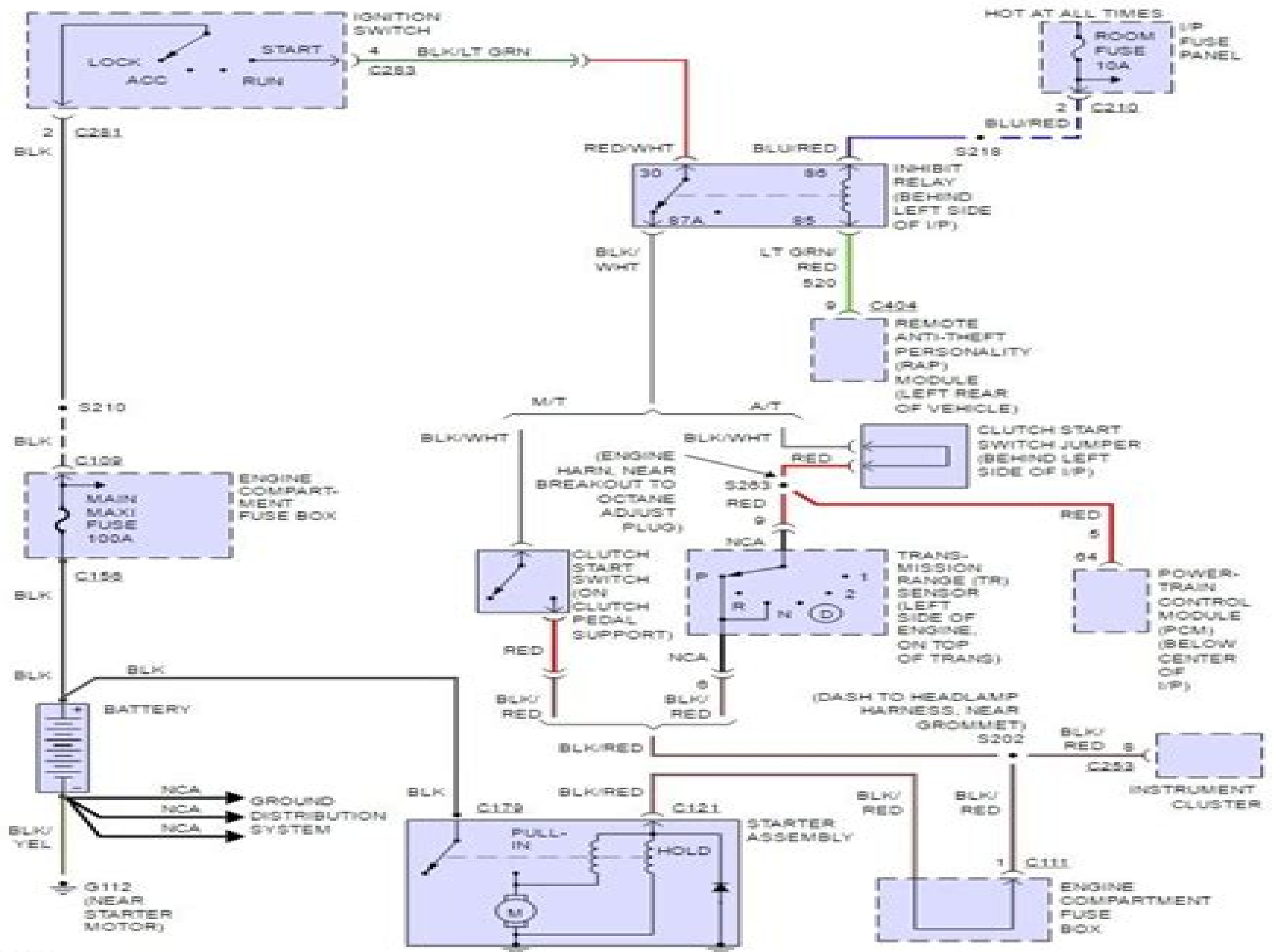
Fig 2 Starting Circuit
