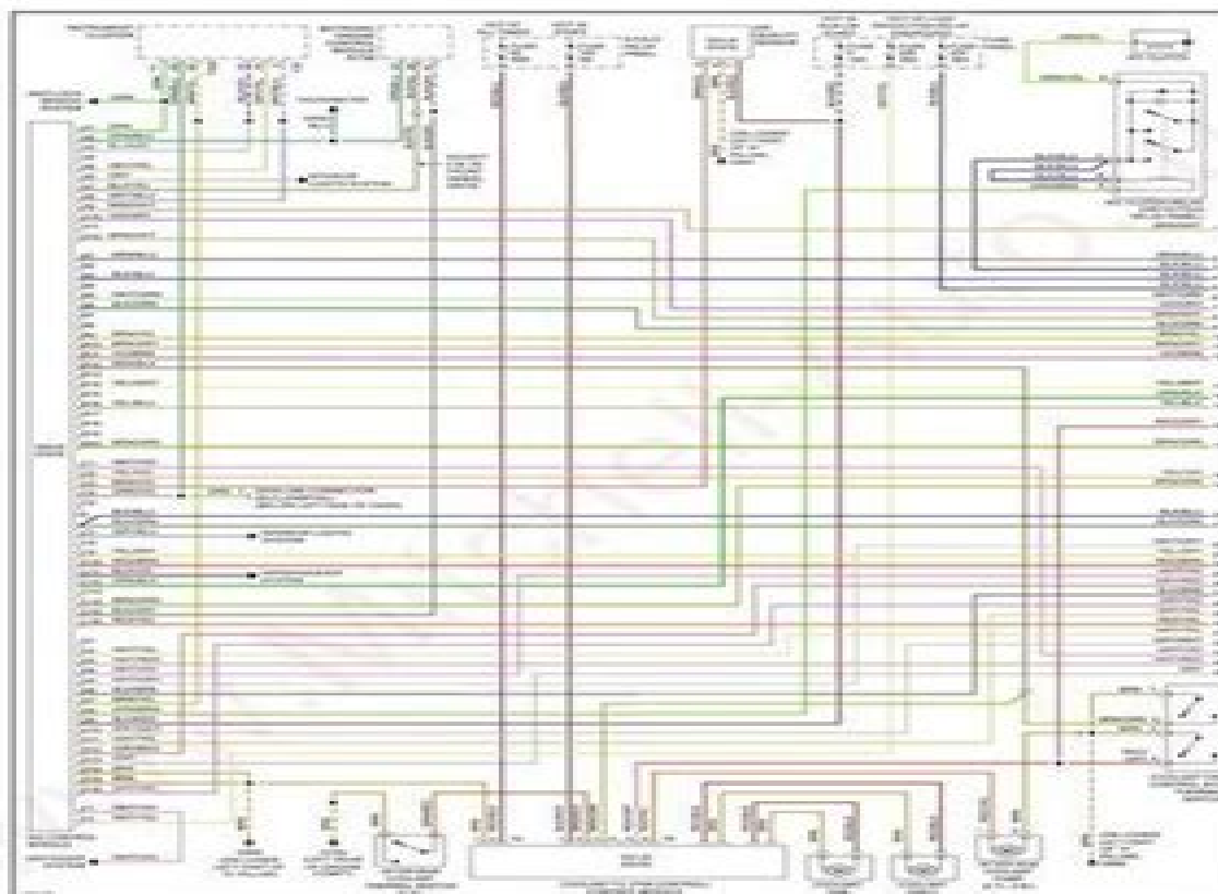
Fig. 1: Automatic A/C Circuit, W/ Coolant Fan Control Module (1 of 2)
