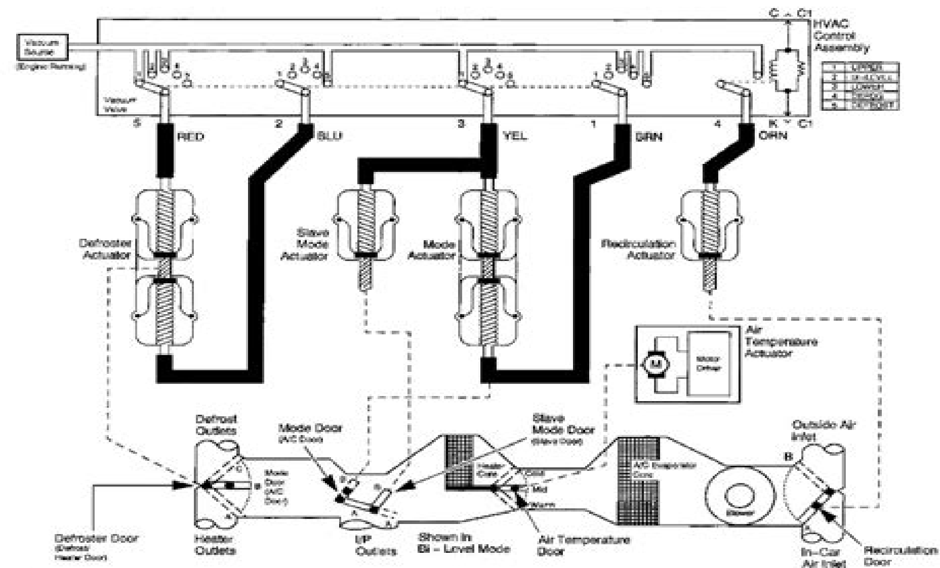
Fig 1: Manual A/C-Heater System Vacuum Diagram (Blazer - Jimmy Canadian, Sonoma & S10 Pickup)
