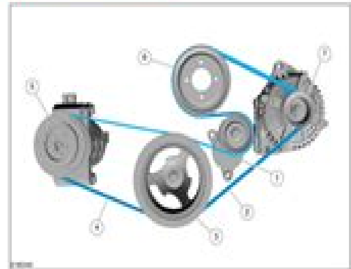
Fig. 1-102 Accessory Drive Belt Routing and Component Location
