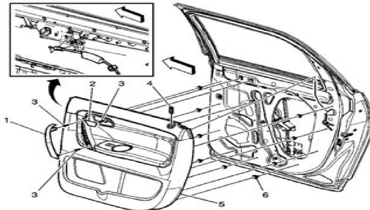
Fig. 4: Identifying Rear Side Door Trim Panel Courtesy of GENERAL MOTORS CORP.
