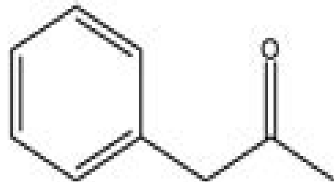
phenyl-2-propanone Molecular Weight: 134,18
