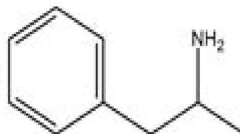
Amphetamine Molecular Weight: 135,21
