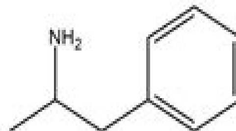
Di 1-Phenylpropan-2-amine sulfate Molecular Weight: 368,49
