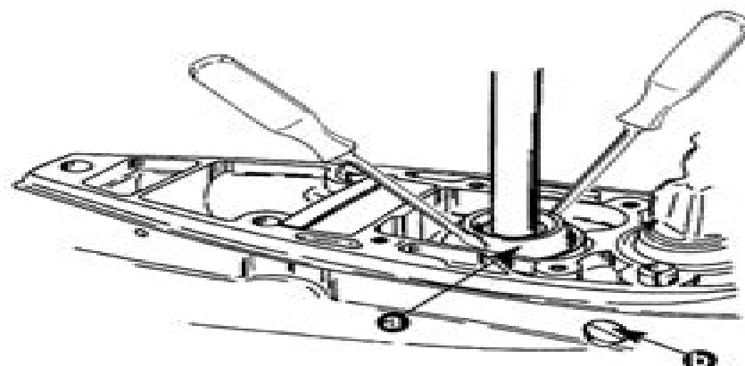
a - Water Pump Base b - Vent Plug
