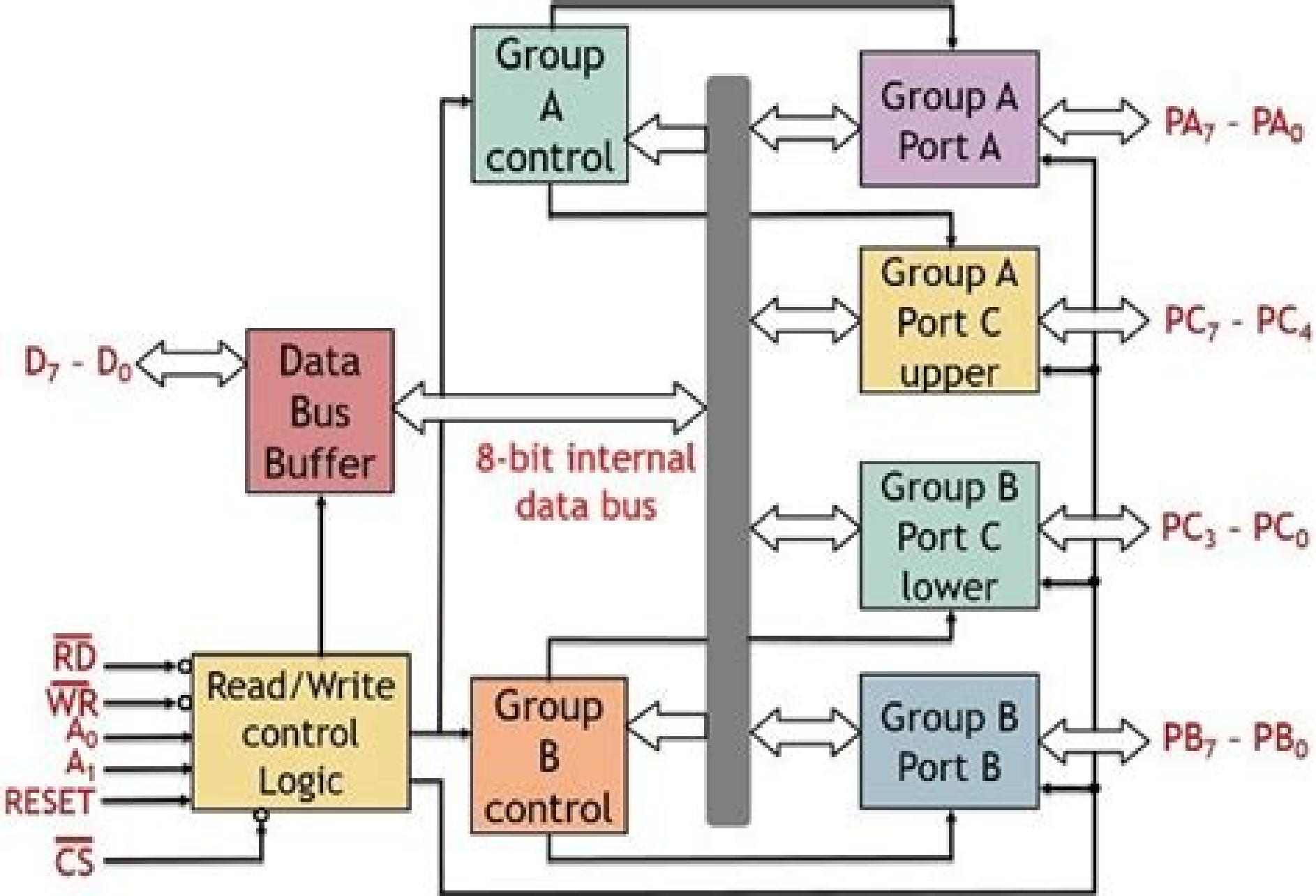
Architecture of 8255 PPI
