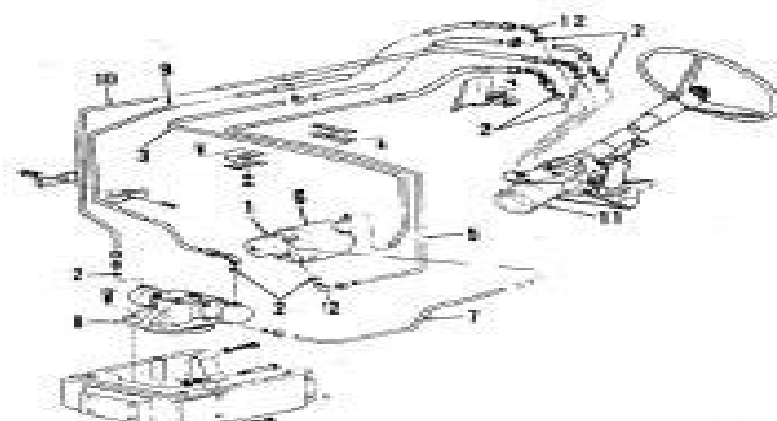
Fig. 5—8000—8000 hydrostatic power steering system with integral hydraulic pump and reservoir. Refer to Fig. 4 for identification of components. Steering motor (11) is pressurized from tube (9) to lower part. Upper part returns fluid through tube (10) to reservoir (6). Tubes (9) and (10) are routed to front steering motor (8) from side parts.
