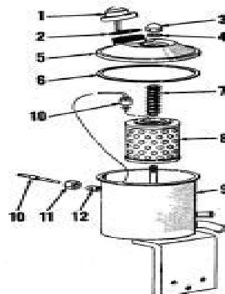
Fig. 6—Exploded view of power steering system reservoir used on 8000 and 8000 models and early 8000 and 8000 models. Oil level switch (10) is connected to warning light on instrument panel. Filter element (8) and oil reservoir should be renewed after each 800 hours of use.
