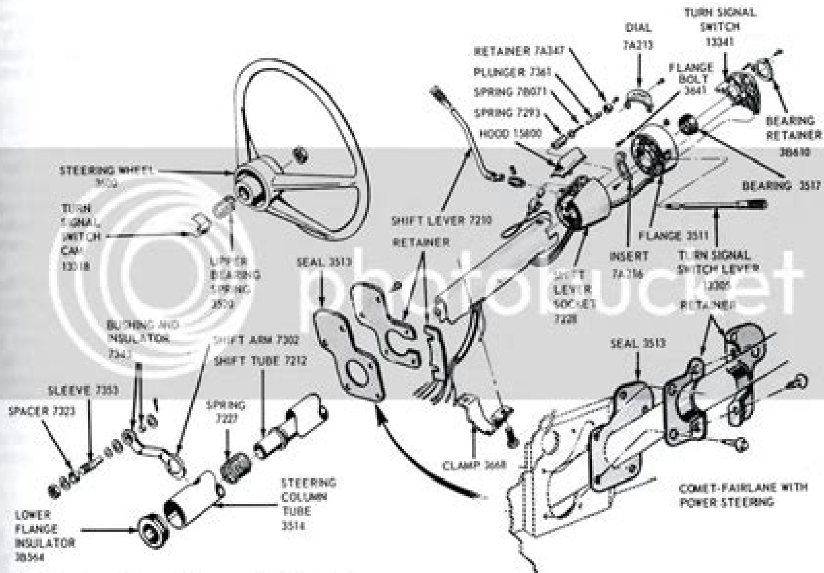
FIG. 6—Steering Column Disassembled—Typical
