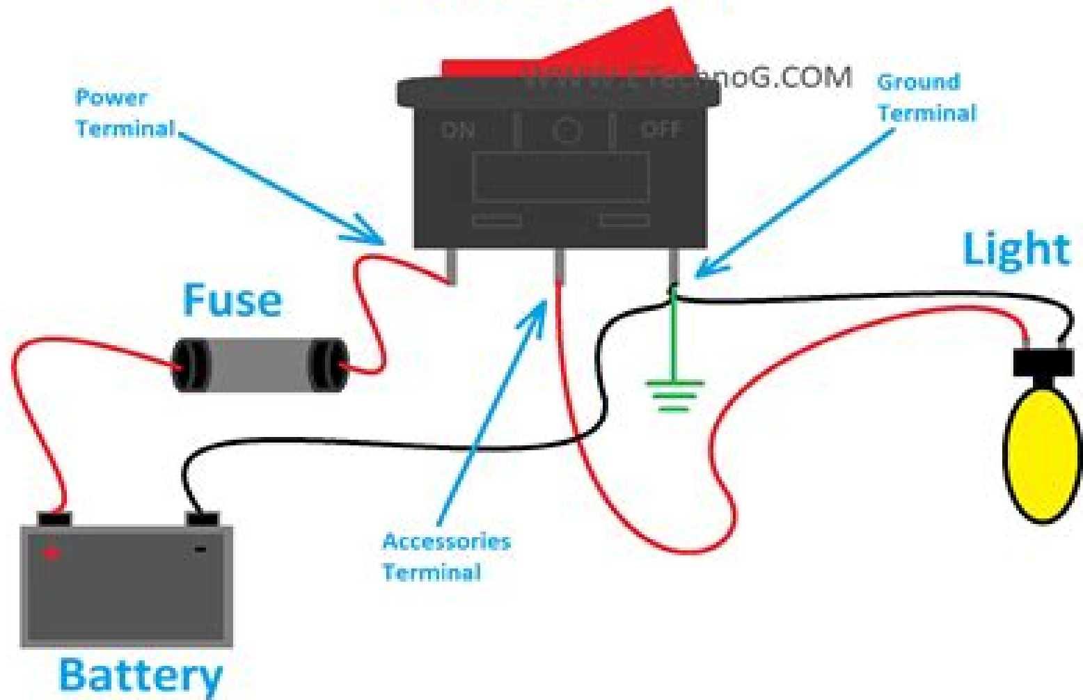
Rocker Switch Wiring and Connection Diagram
