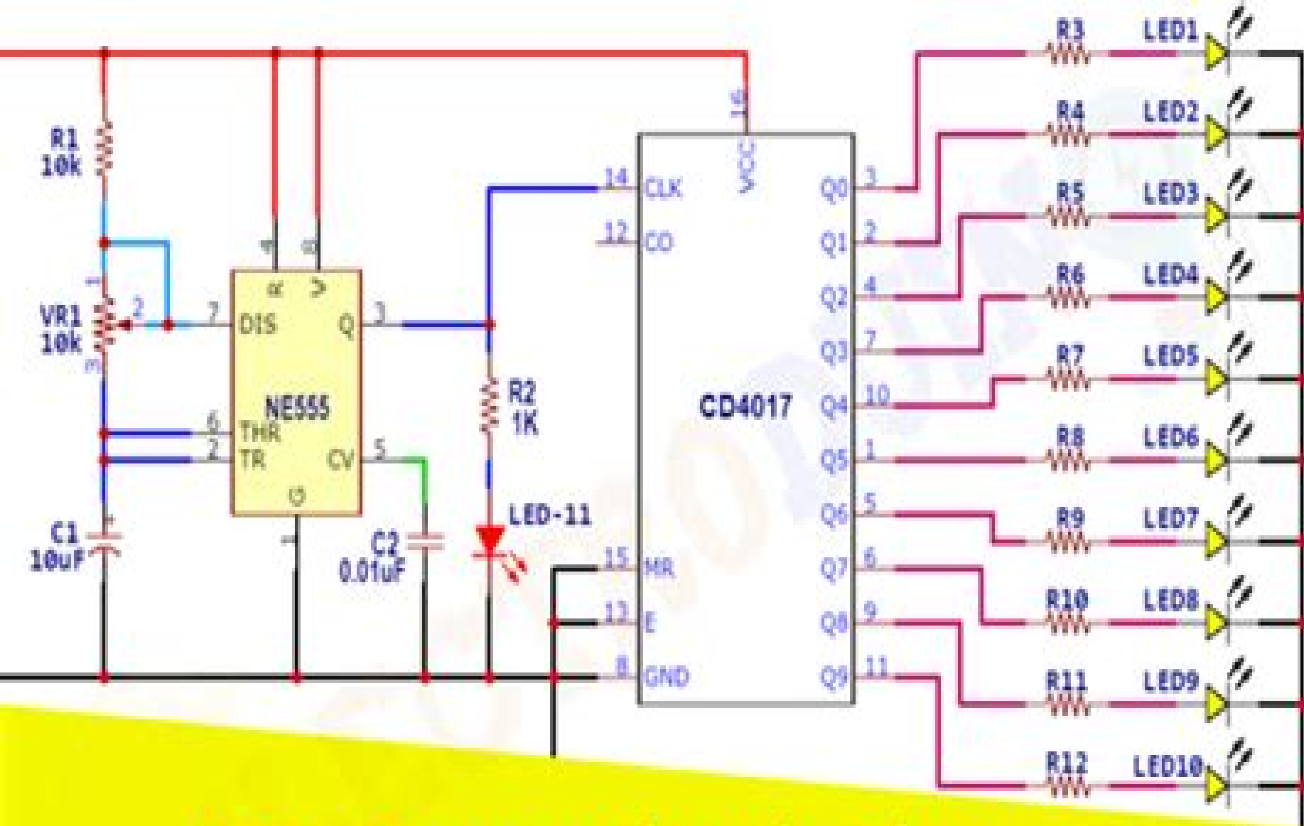
LED Chaser Circuit Diagram Running Light
