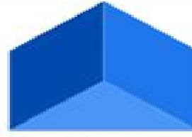
Triangular prism
