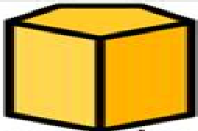
pentagonal prism
