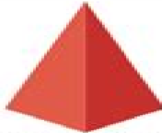
3D pyramid
