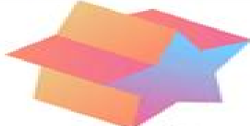
star prism
