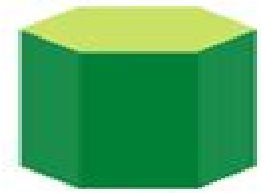
Hexagonal prism
