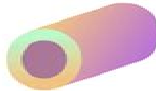
hallow cylinder
