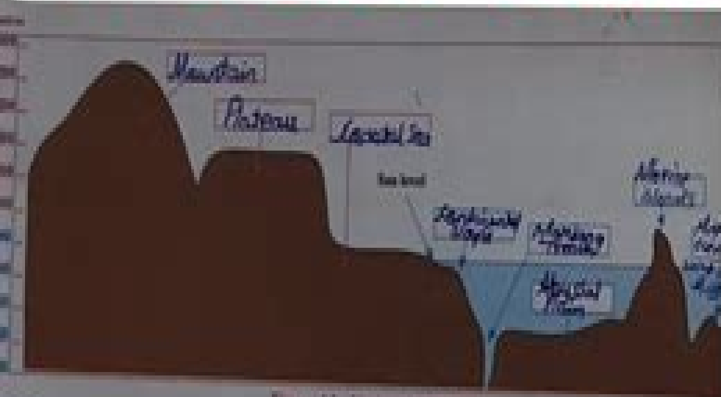
Figure 4.1 : Various landforms
