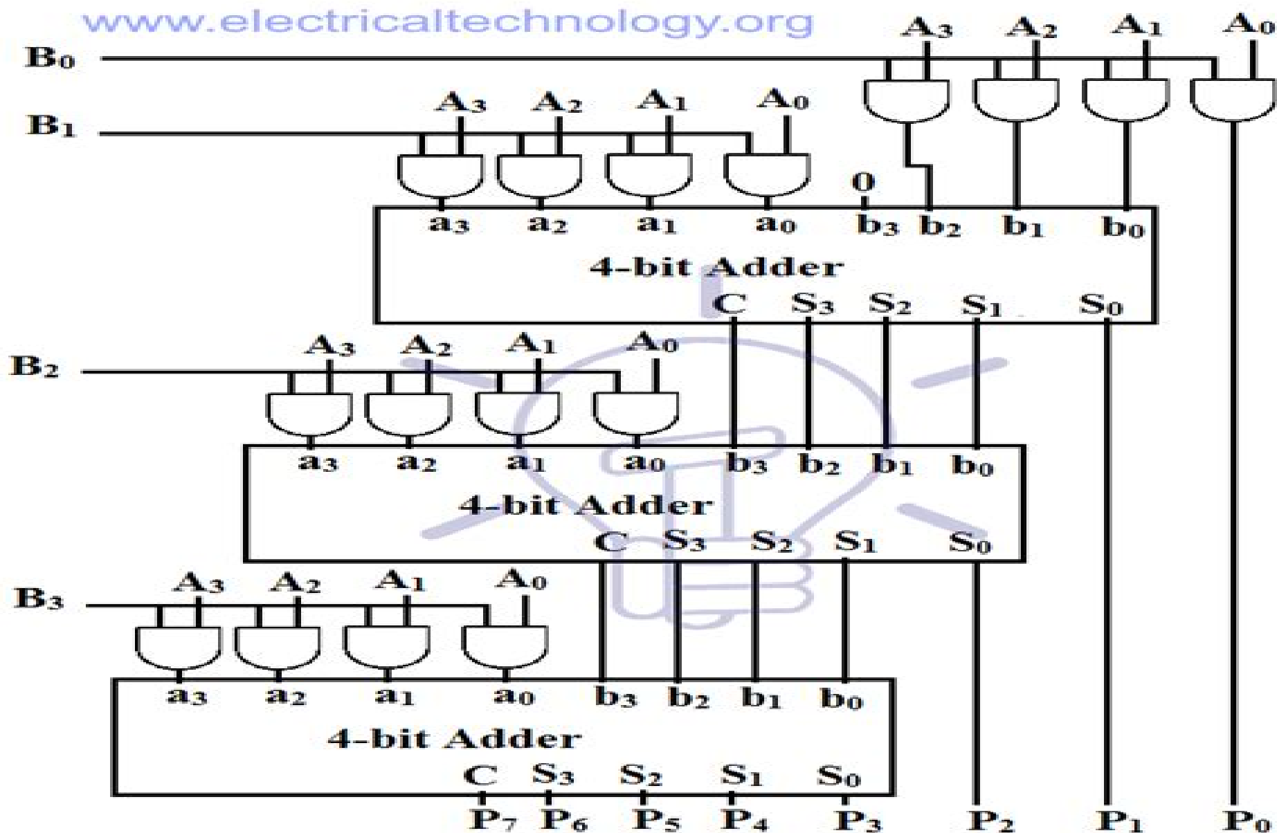
Schematic of 4x4 Multiplier Using 4-Bit Full Adders
