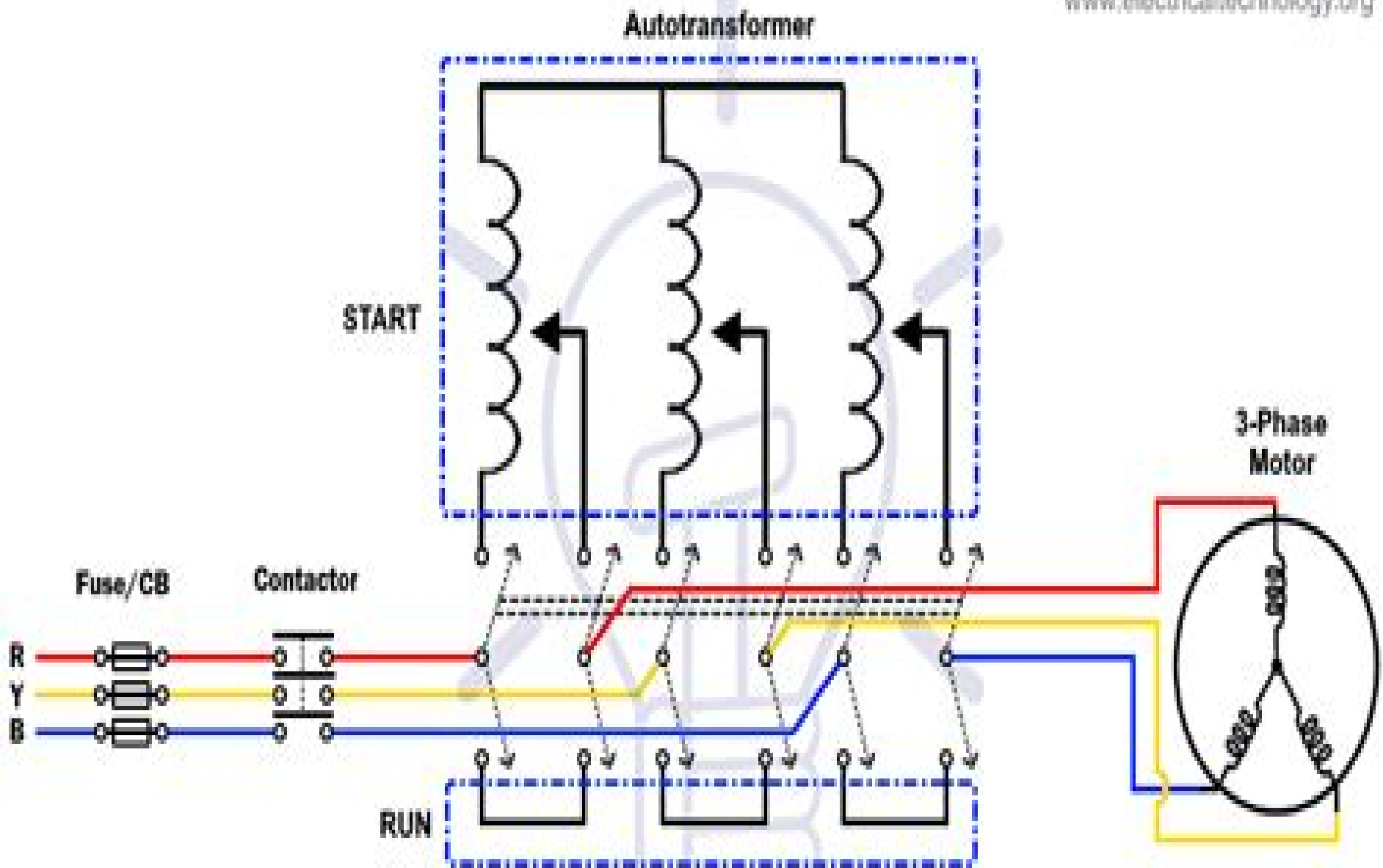
Autotransformer Motor Starter
