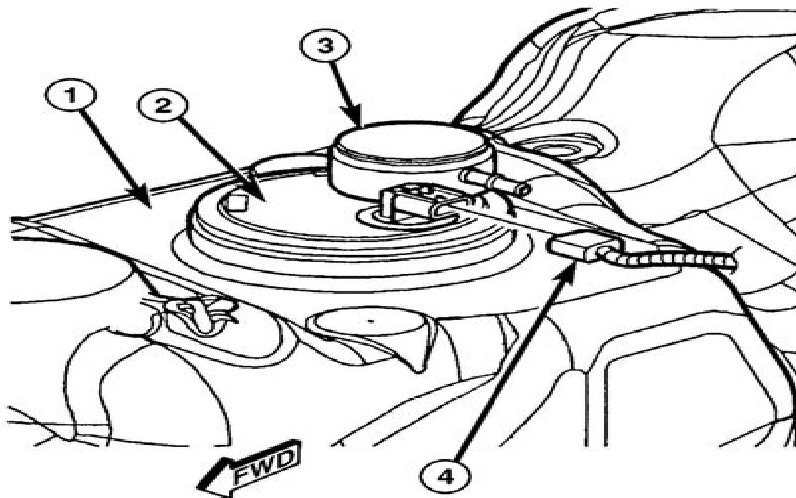
Fig. 30 FUEL PUMP MODULE CONNECTIONS
