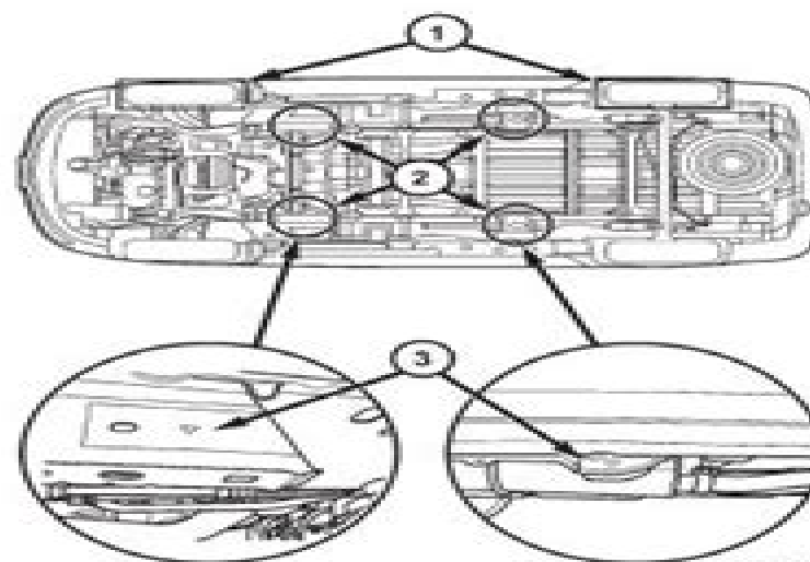
Fig. 8 HOISTING AND JACKING POINTS
