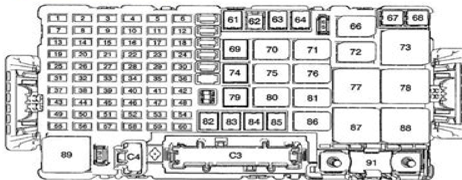
Fig 23: Underhood Fuse Block
