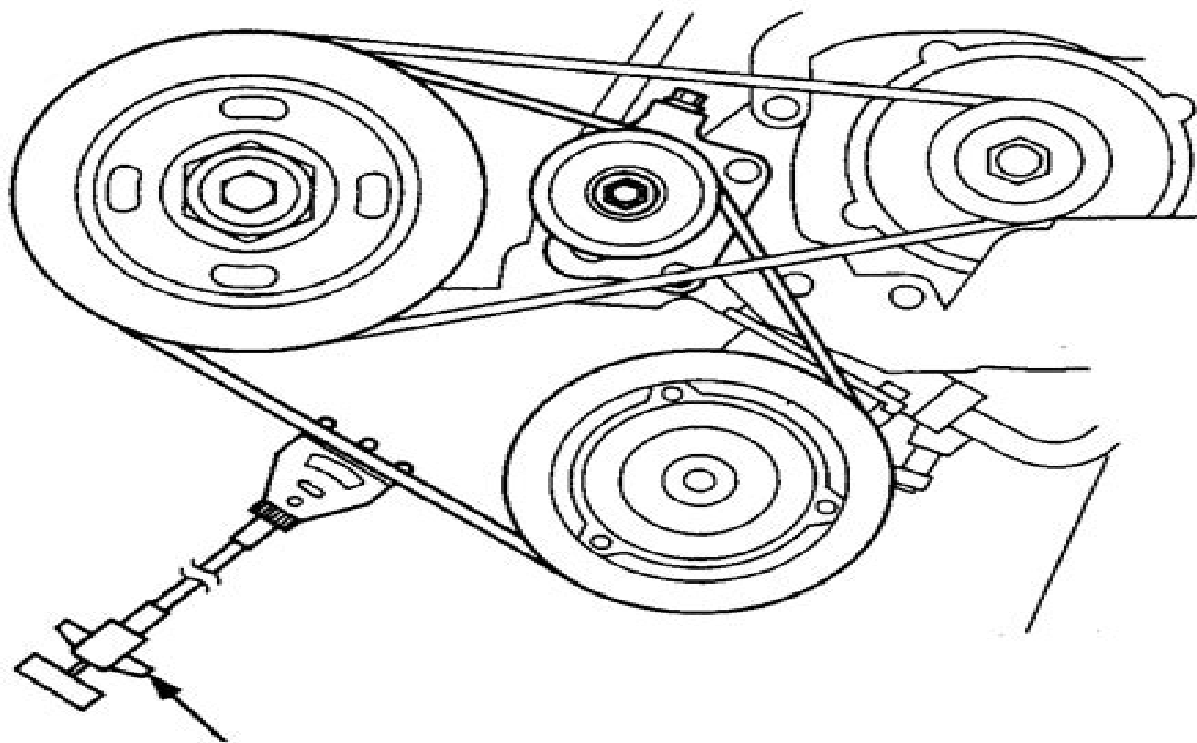
BELT TENSION GAUGE 07JGG - 001010A
