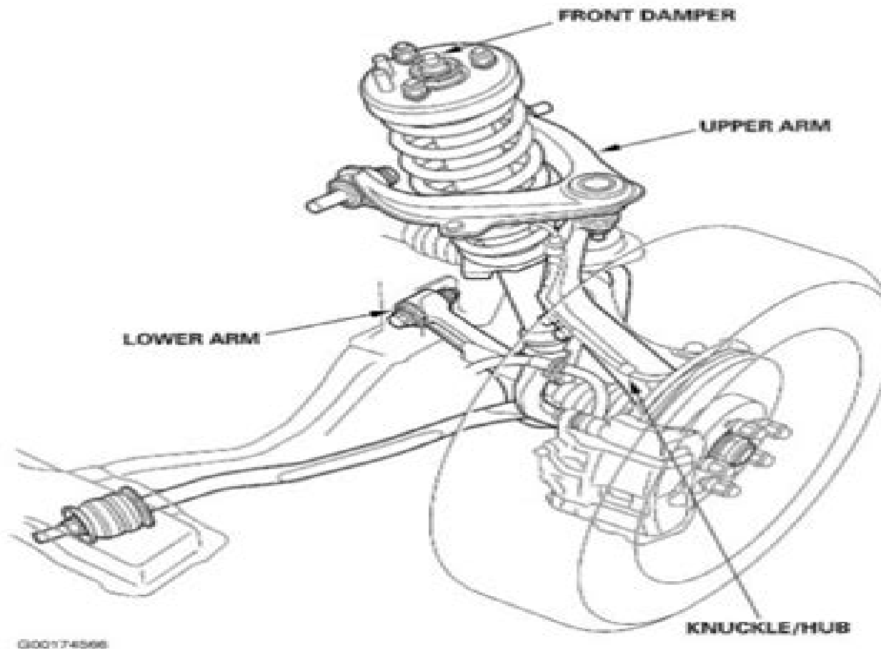
Fig. 1: Locating Components Courtesy of AMERICAN HONDA MOTOR CO., INC.
