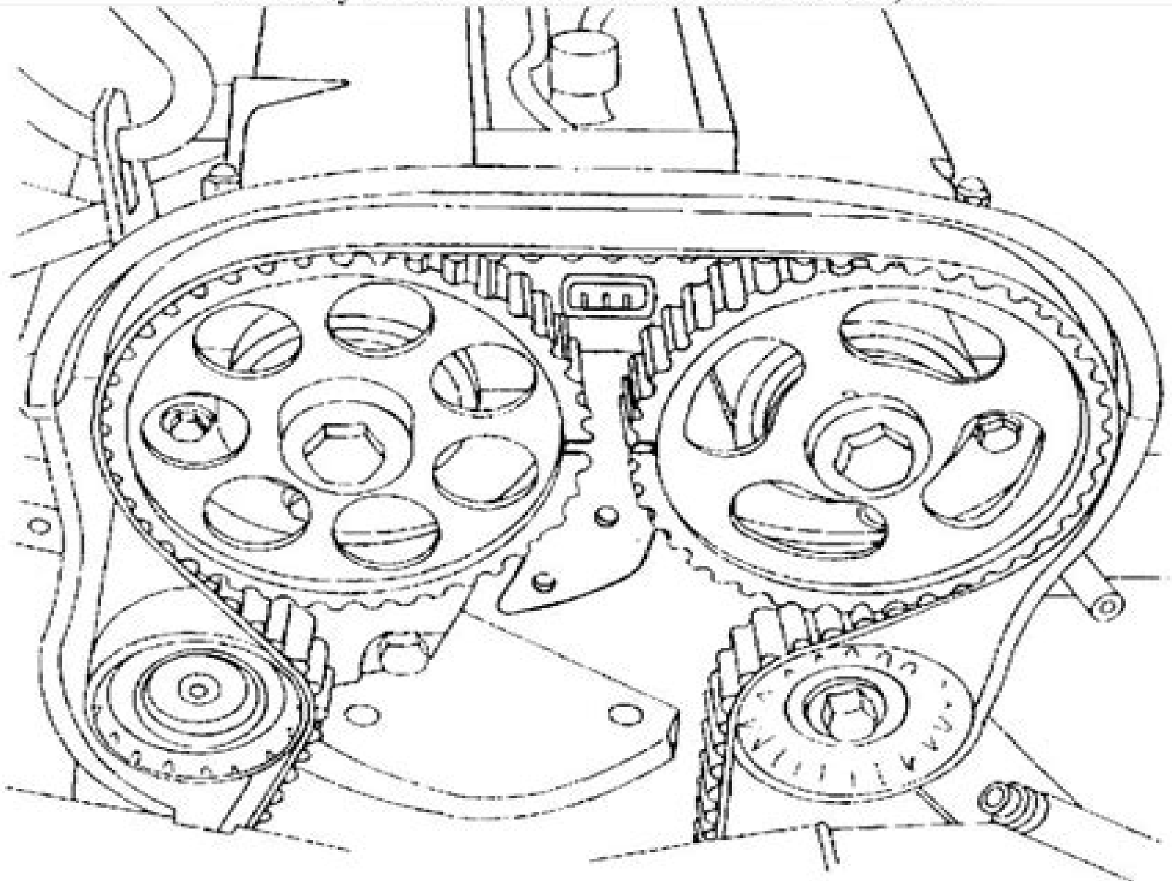
Fig. 4: Aligning Camshaft Sprocket Timing Marks Courtesy of DAEWOO MOTOR AMERICA, INC.
