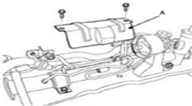
Fig. 16: Identifying Heat Protector Courtesy of KIA MOTORS AMERICA, INC.
