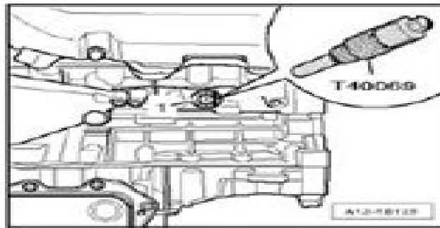
Fig. 335: Securing Crankshaft Hole For T40069 Into the
