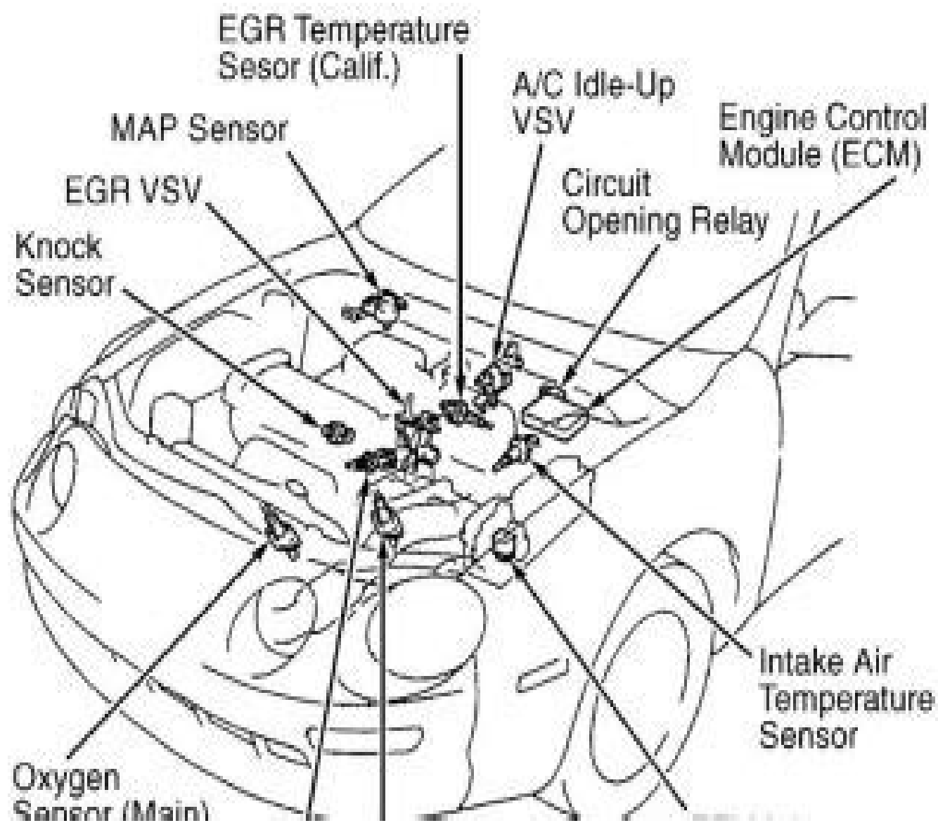
Fig. 1: Component Locations (1 Of 4)
