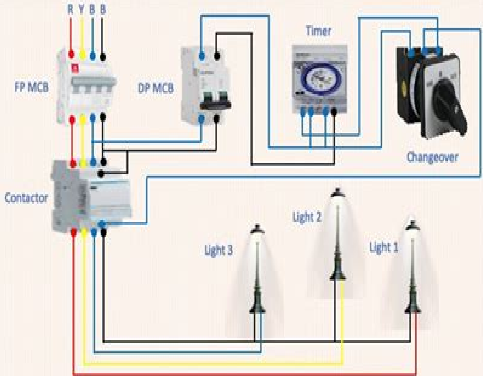
3 phase pole lighting wiring Diagram
