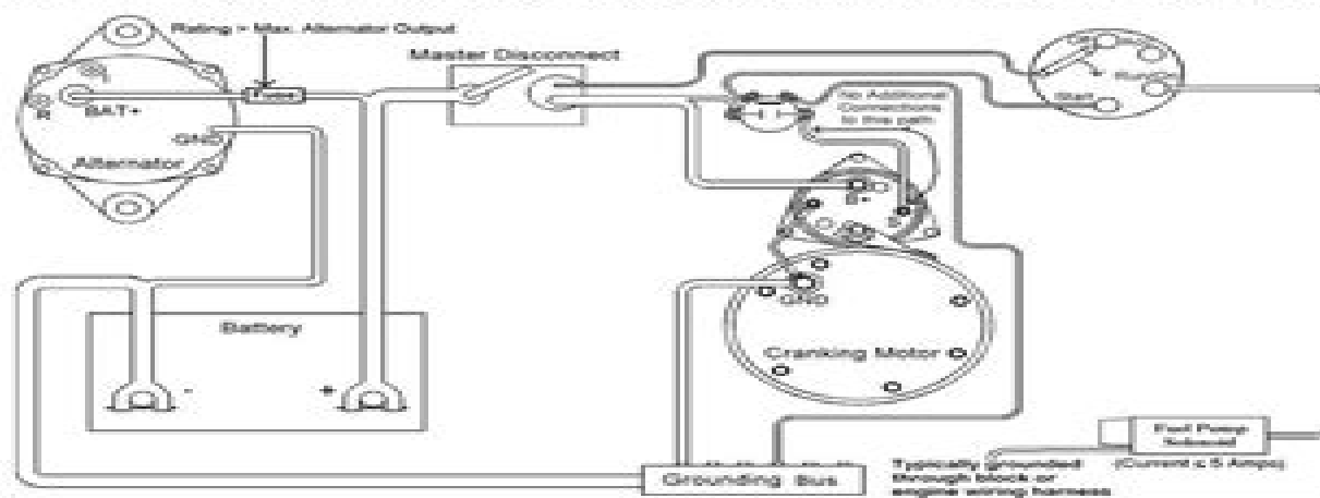
Figure 3.6 Low Current Fuel Shut-Off Solenoid (acceptable wiring method for current draw \leq 5 A)
