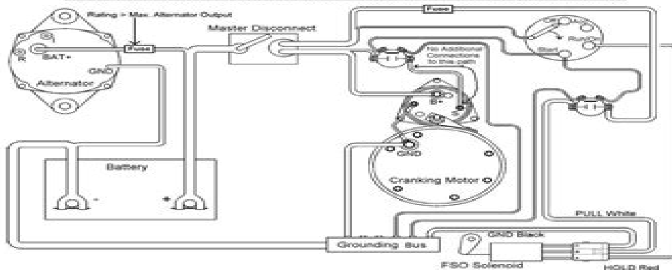
Figure 3.5 Two Relay Shutdown/Starting System (Preferred Method)
