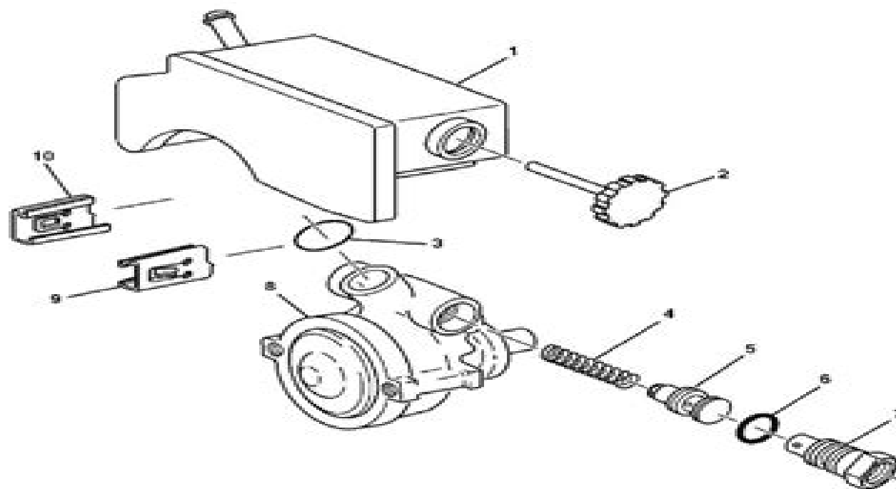
Fig. 2: Exploded View Of Power Steering Pump Components (CB Series) Courtesy of GENERAL MOTORS CORP.
