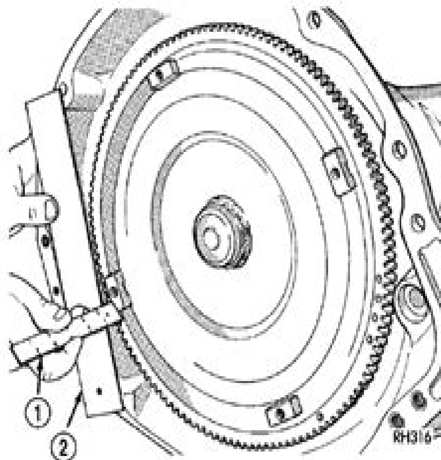
Fig. 33: Checking Torque Converter Seating
