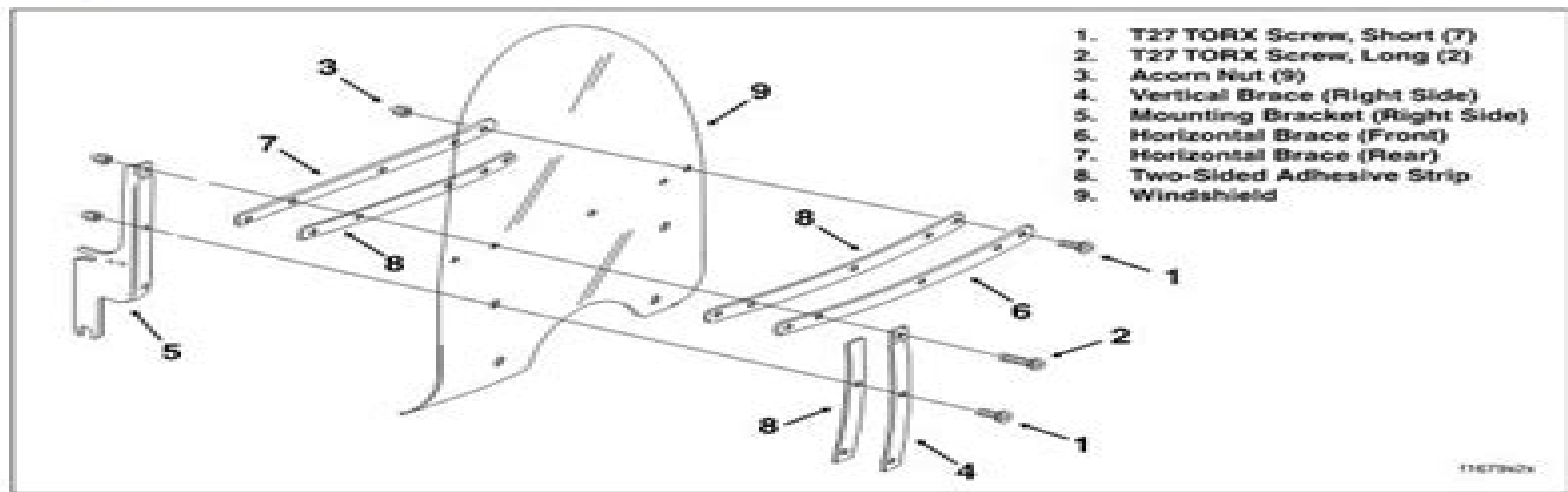
Figure 2-190. Windshield Assembly
