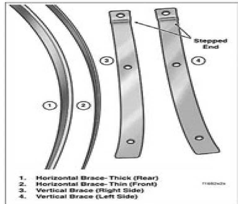
Figure 2-191. Windshield Braces
