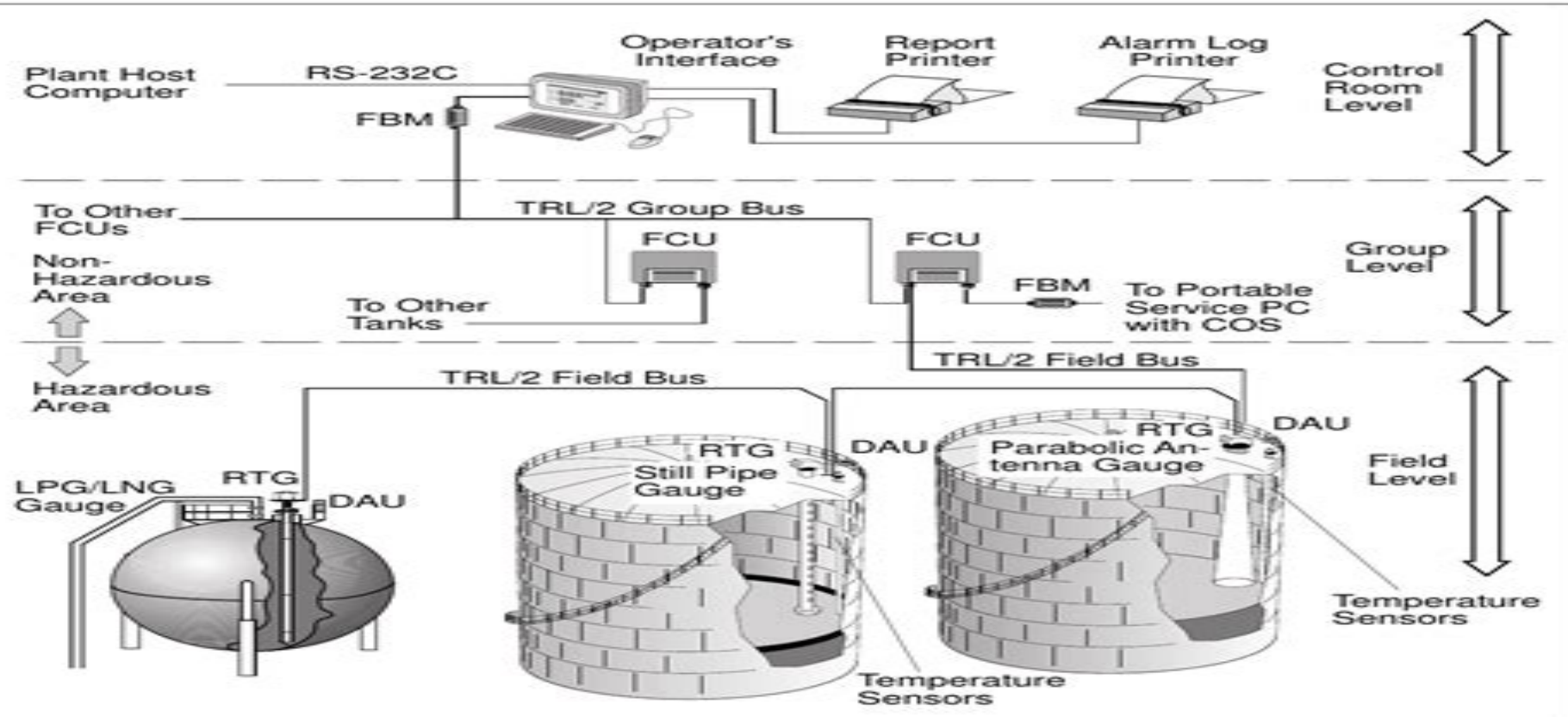
Figure 1.2. Example of a general configuration of a TankRadar L/2 System.
