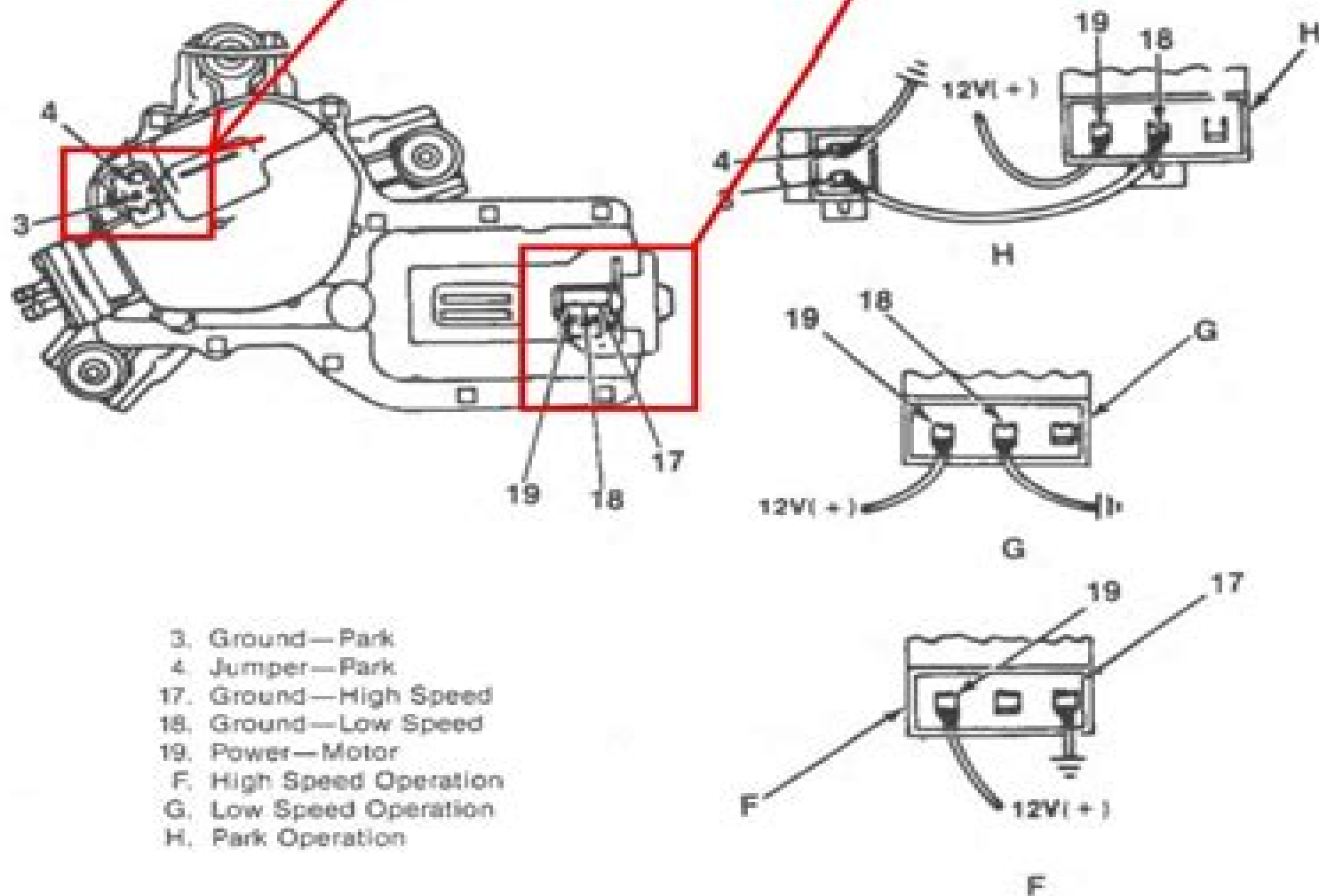
Figure 30—Diagnosis Connections
