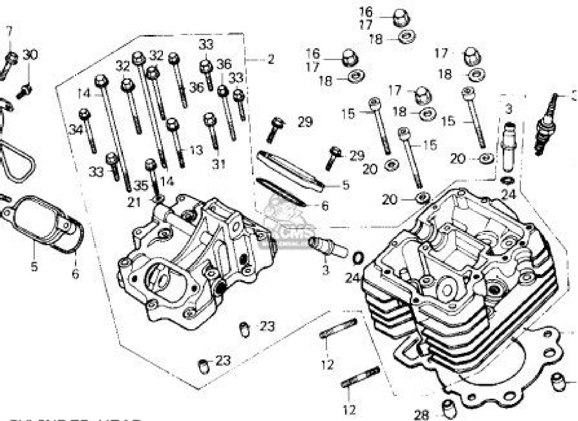
CYLINDER HEAD
