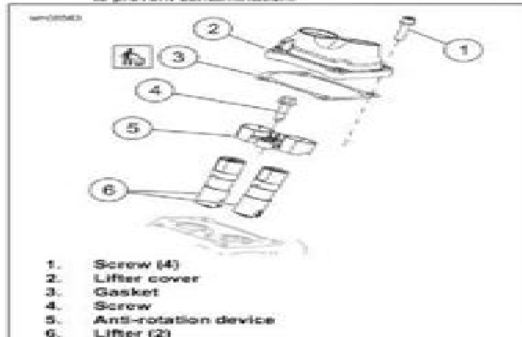
Figure 4-25. Lifter Cover
