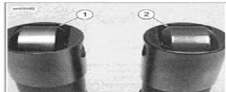
1. Normal roller 2. Frosted roller Figure 4-26. Roller Inspection
