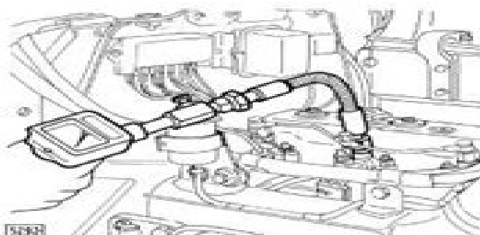
Checking engine compression using tester 291309.
