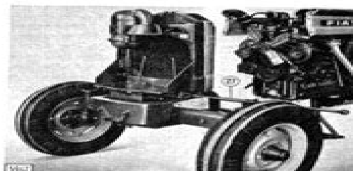
Removing (installing) from axle (640).
