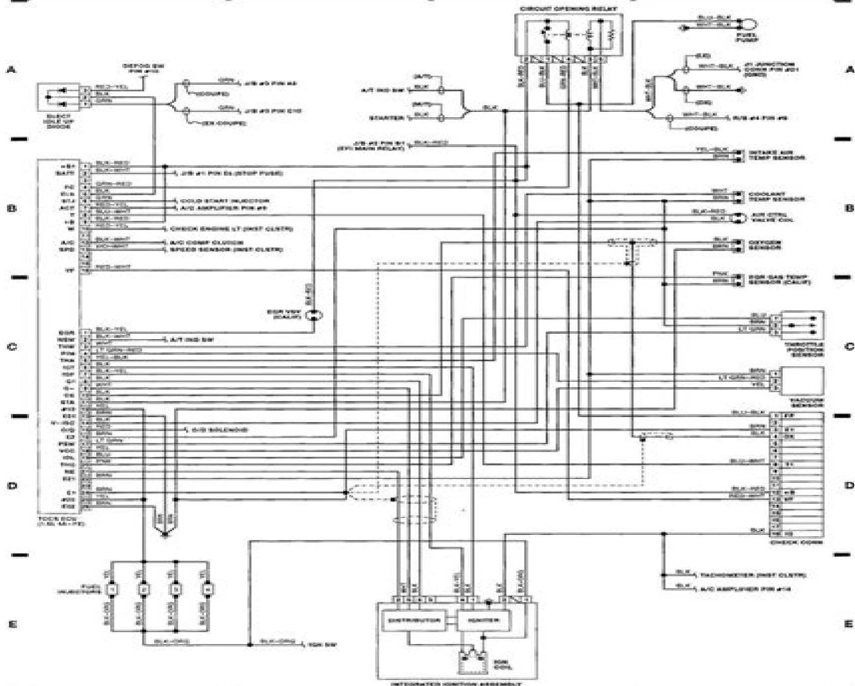
Fig. 2: Computer Engine Control (1.6L 4A-FE) (Grid 4-7)
