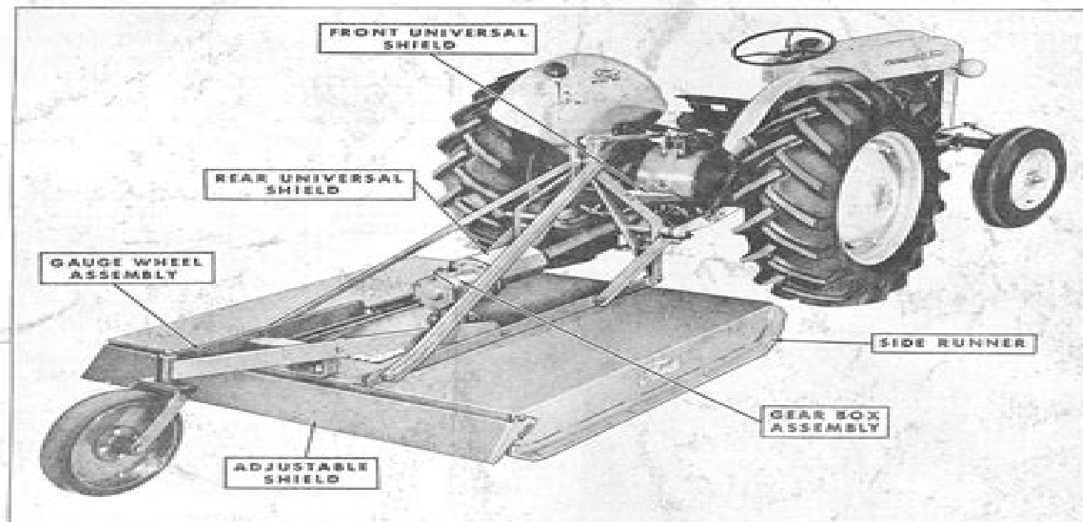
Figure 1 60" Rotary Cutter Installed
