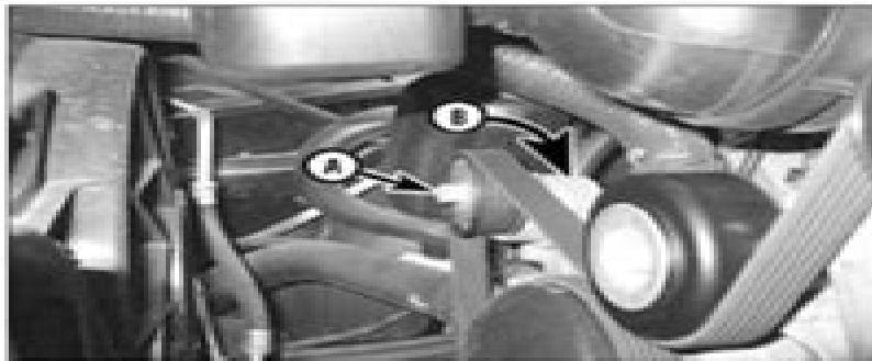
12.5a Place a socket on the tensioner bolt (A) and turn the tensioner clockwise (B) for belt removal
